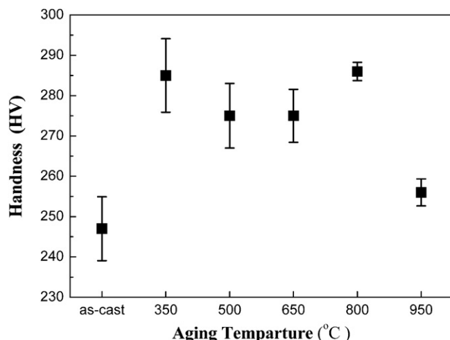
Fig. 1. Hardness of Al 0.5 CoCrFeNi alloy processed at various aging temperatures.
